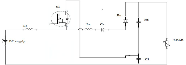
Fig 5.operating mode 4
