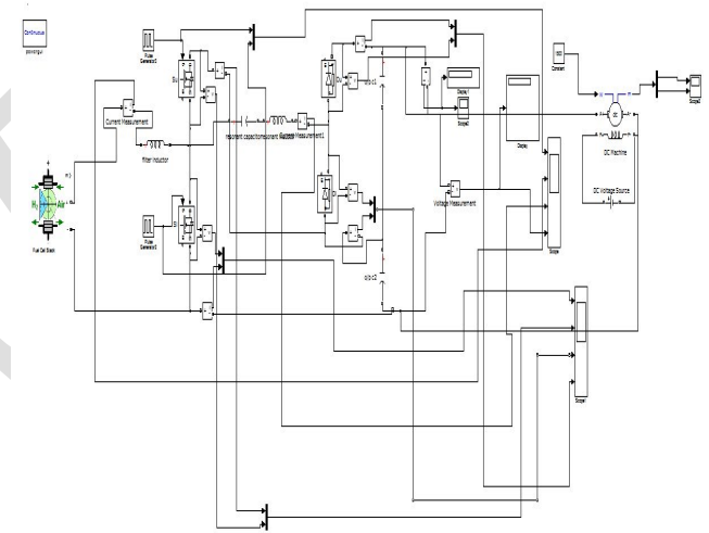
Fig 16. Simulation diagram of fuel cell fed resonant PWM converter fed PMDC motor
