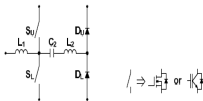
Fig 20. Basic cell
