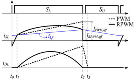
Fig 7. Comparison of switch and diode current waveforms.
