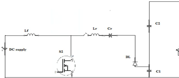
Fig 3.operating mode 2
