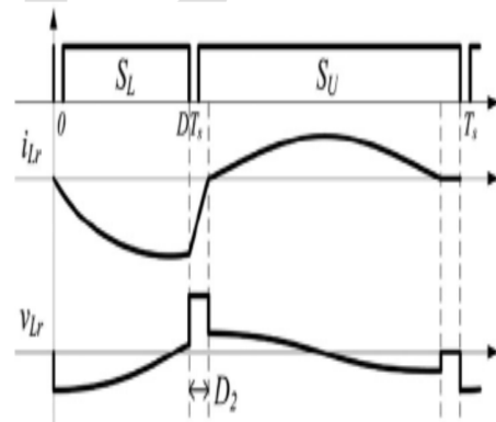
Fig 12 . Above resonance operation with D < 1 - (f_s/2f_r)
