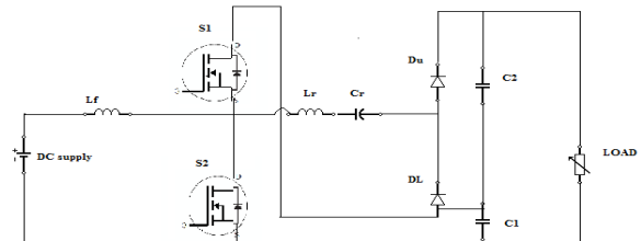
Fig 1. Proposed converter
