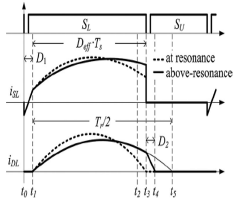
Fig 9. Comparison of switch and diode current waveforms of two resonant condition.
