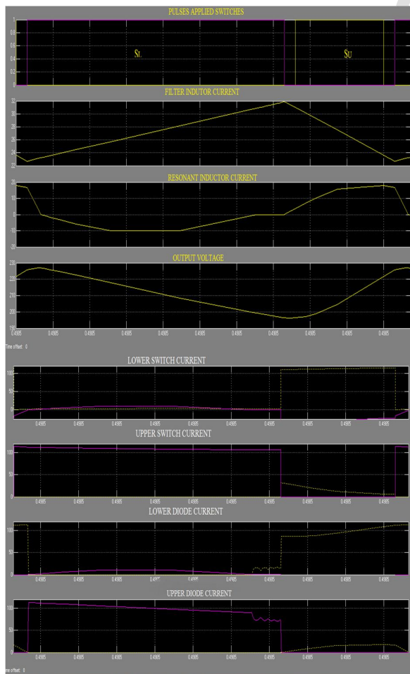
Fig 14. Output waveforms of proposed converter
