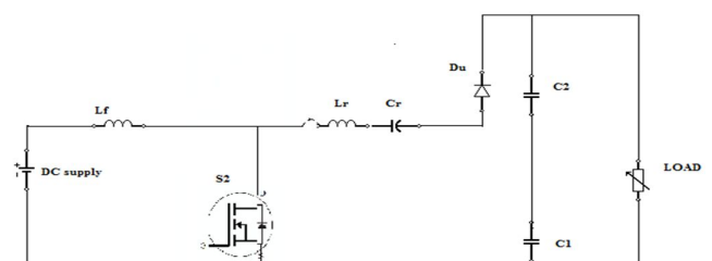
Fig 2. operating mode 1
