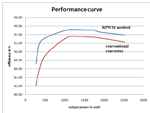
Fig 19. Comparison of performance curve.
