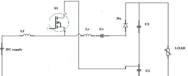
Fig 6.operating mode 5
