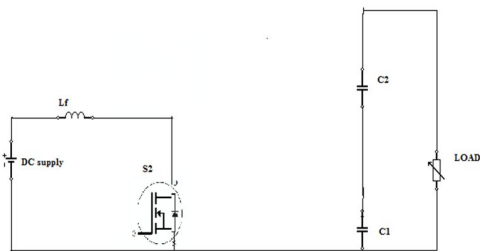
Fig 4.operating mode 3
