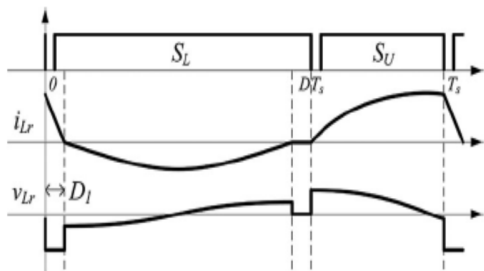
Fig 10 . below resonant operation with D > f_s/2f_r
