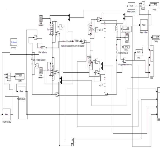
Fig 13. Simulation diagram of proposed converter.
