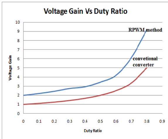
Fig 18. Comparison of voltage gain
